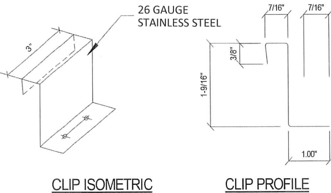
3" Panel Clip Profile
